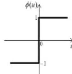
sign function
