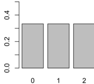
Distribution Q Uniform with p = 1/3
