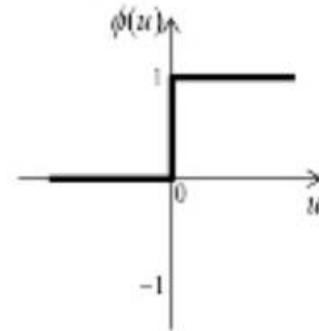
step function
