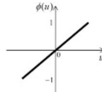
identity function
